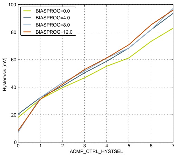
Hysteresis
